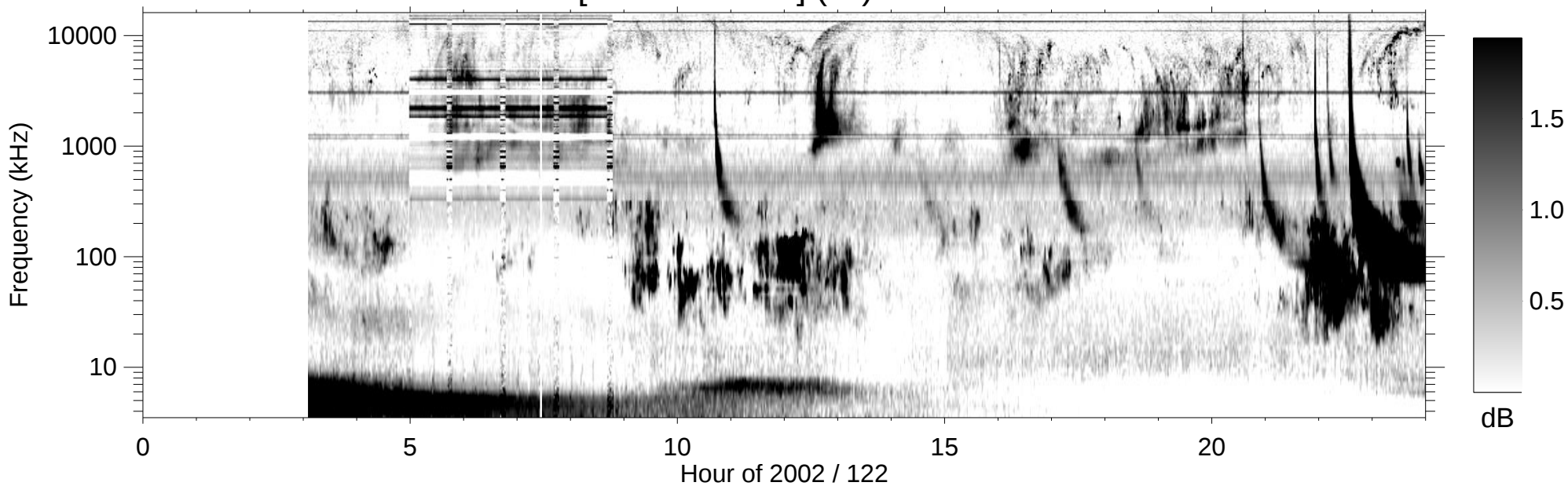
RPWS [ABCH1H2/Ex] (-B) 2002/05/02
