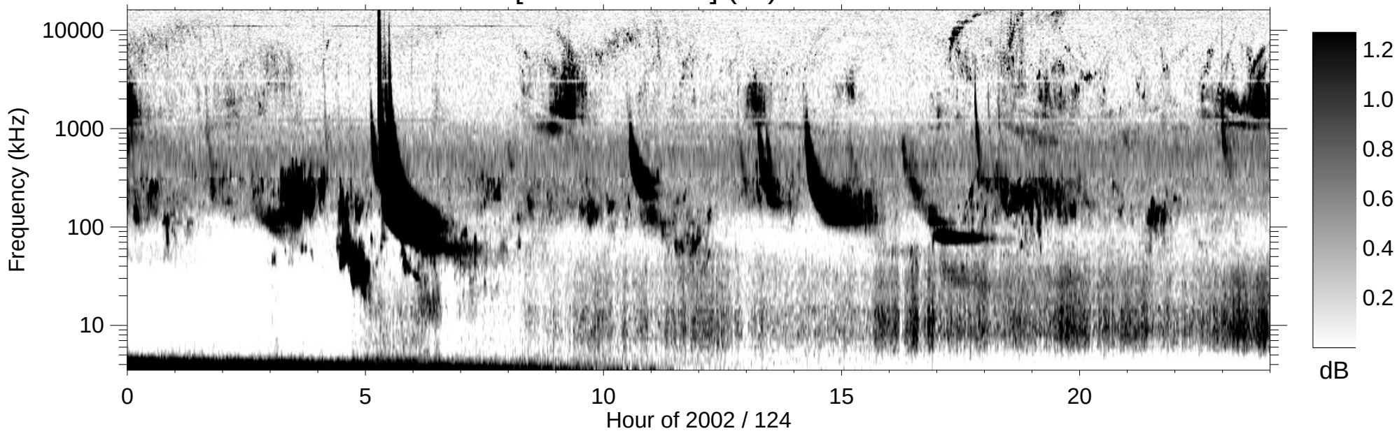
RPWS [ABCH1H2/Ex] (-B) 2002/05/04
