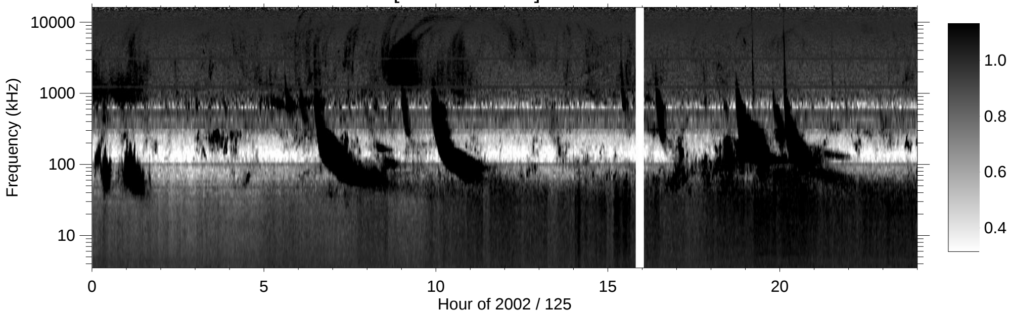
RPWS [ABCH1H2/Ex] (-B) 2002/05/05
