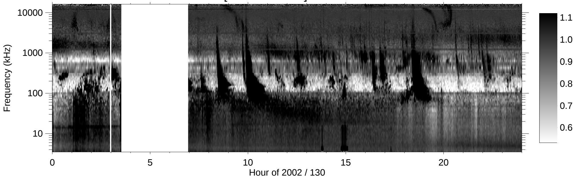
RPWS [ABCH1H2/Ex] (-B) 2002/05/10
