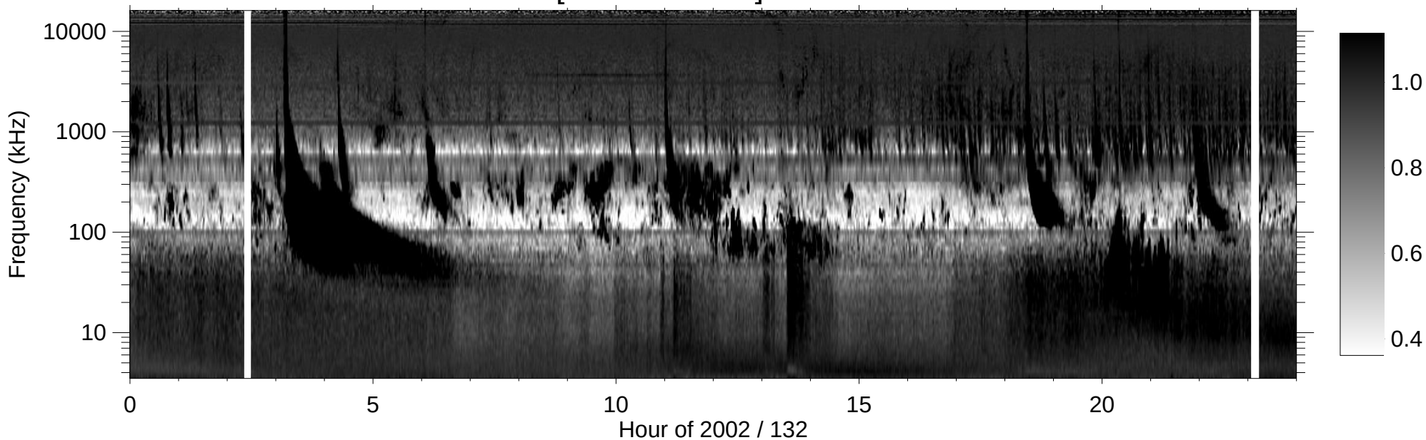
RPWS [ABCH1H2/Ex] (-B) 2002/05/12
