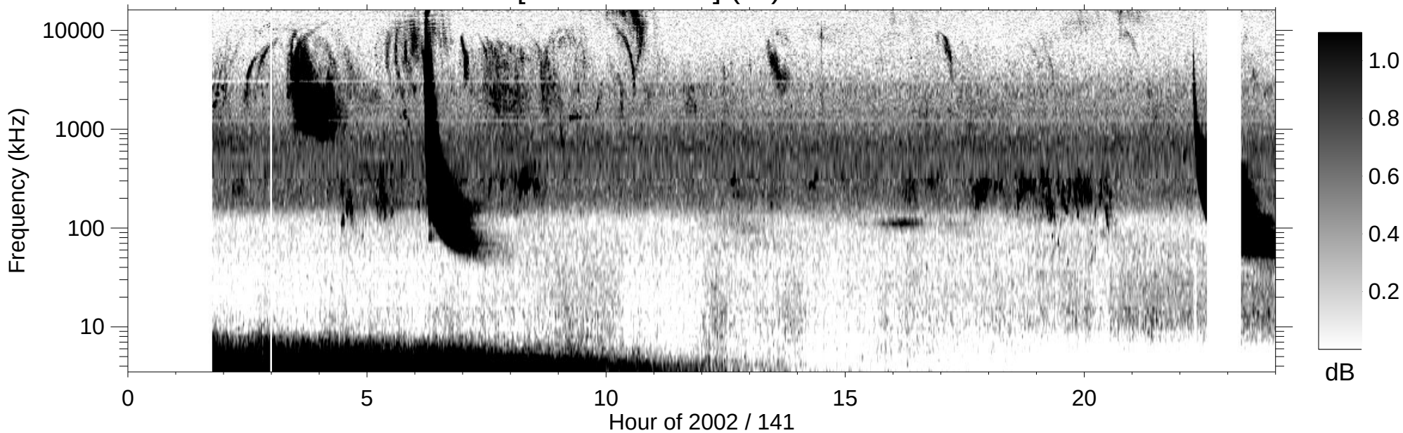
RPWS [ABCH1H2/Ex] (-B) 2002/05/21
