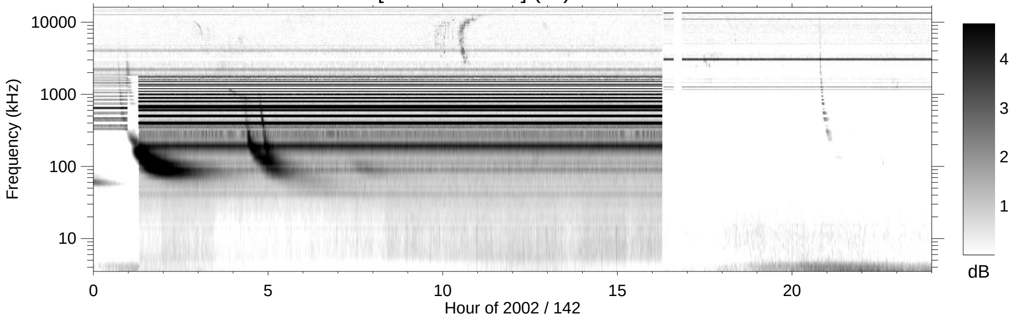
RPWS [ABCH1H2/Ex] (-B) 2002/05/22
