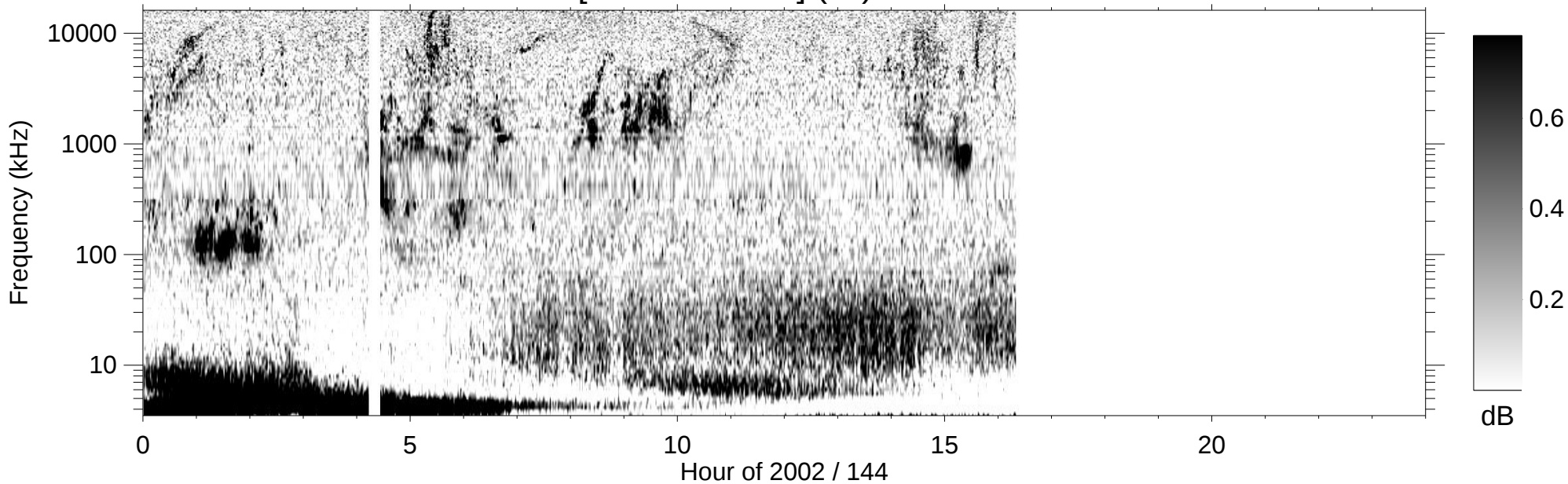
RPWS [ABCH1H2/Ex] (-B) 2002/05/24
