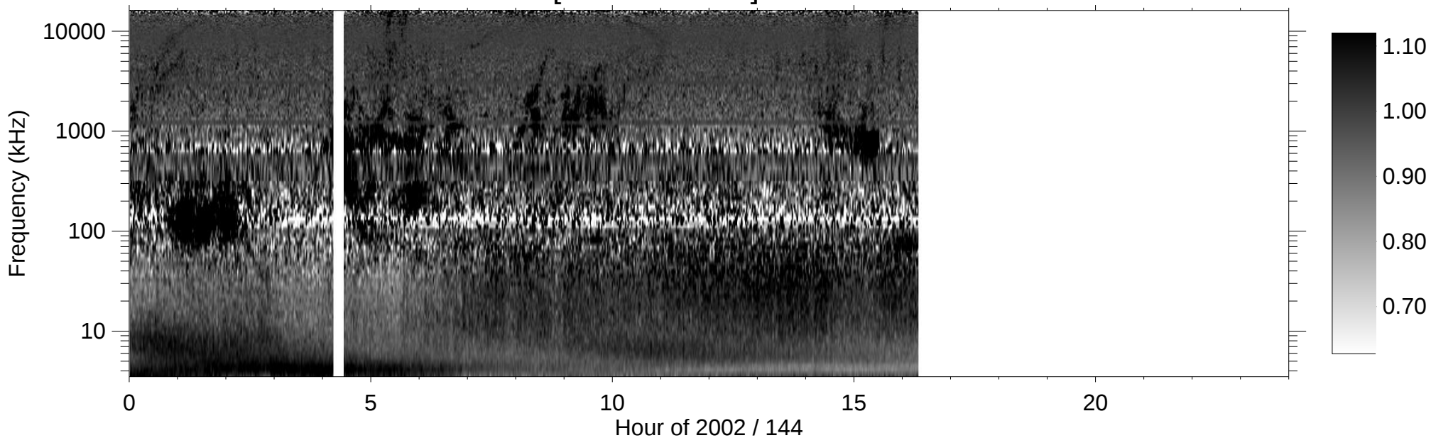
RPWS [ABCH1H2/Ex] (-B) 2002/05/24
