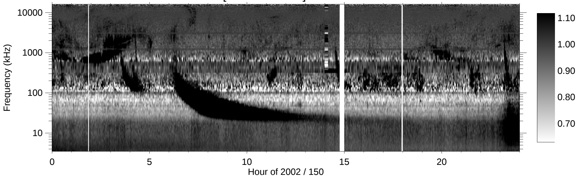
RPWS [ABCH1H2/Ex] (-B) 2002/05/30
