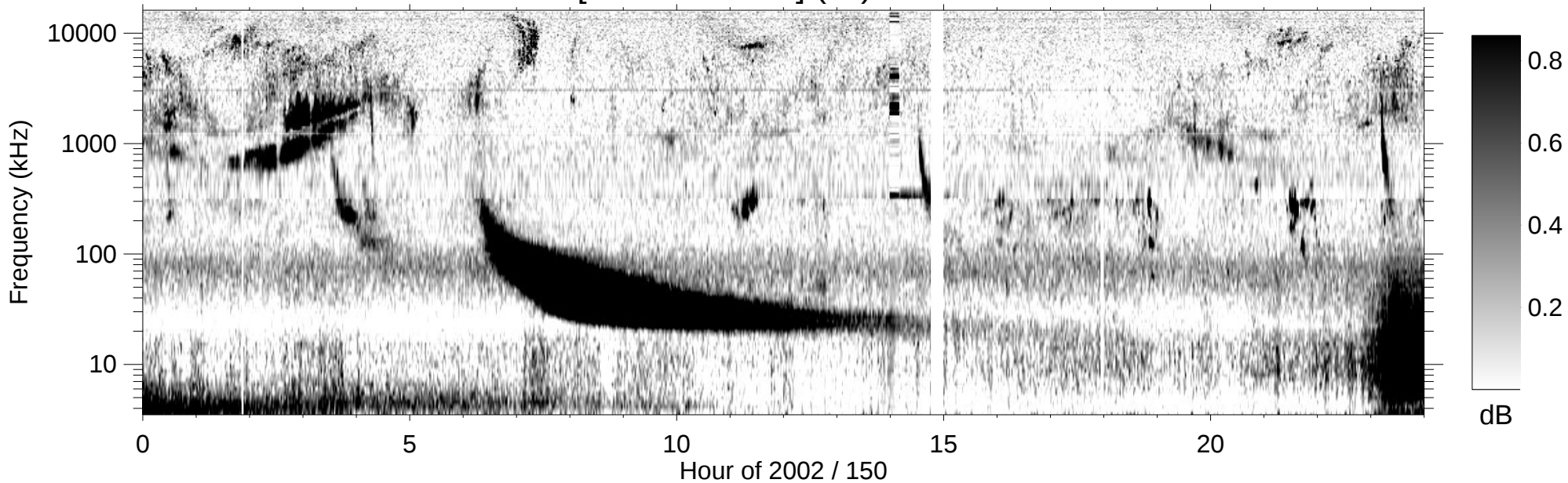
RPWS [ABCH1H2/Ex] (-B) 2002/05/30
