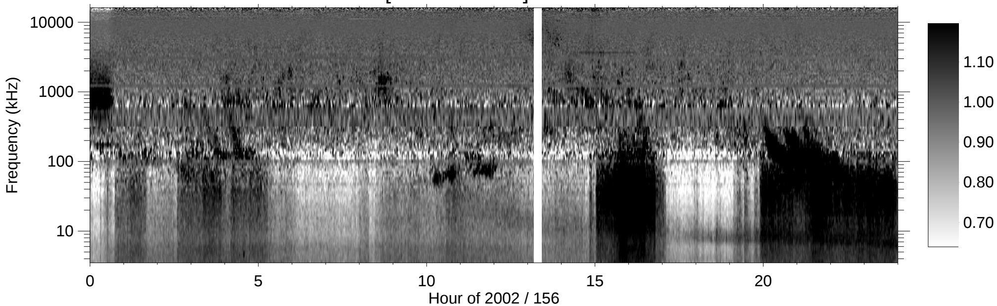
RPWS [ABCH1H2/Ex] (-B) 2002/06/05
