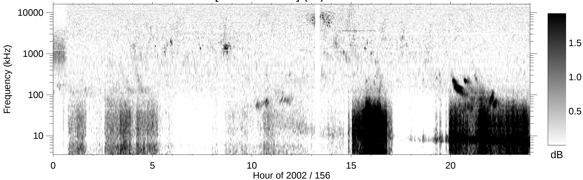
RPWS [ABCH1H2/Ex] (-B) 2002/06/05
