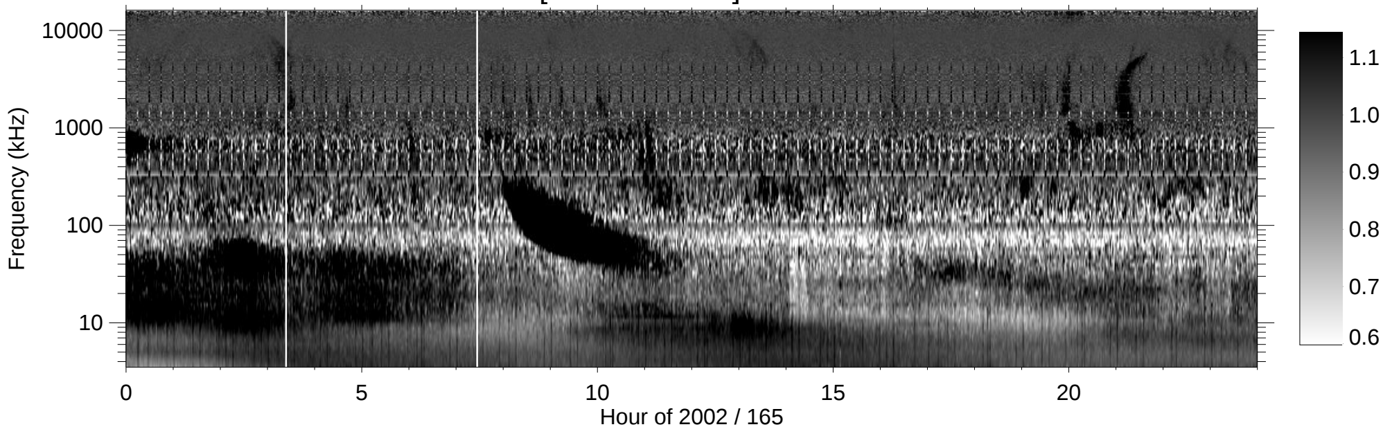
RPWS [ABCH1H2/Ex] (-B) 2002/06/14
