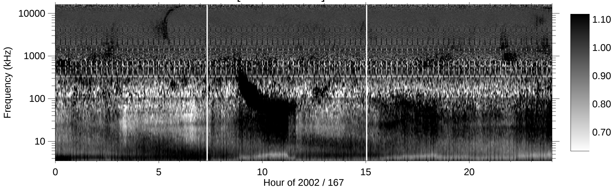
RPWS [ABCH1H2/Ex] (-B) 2002/06/16
