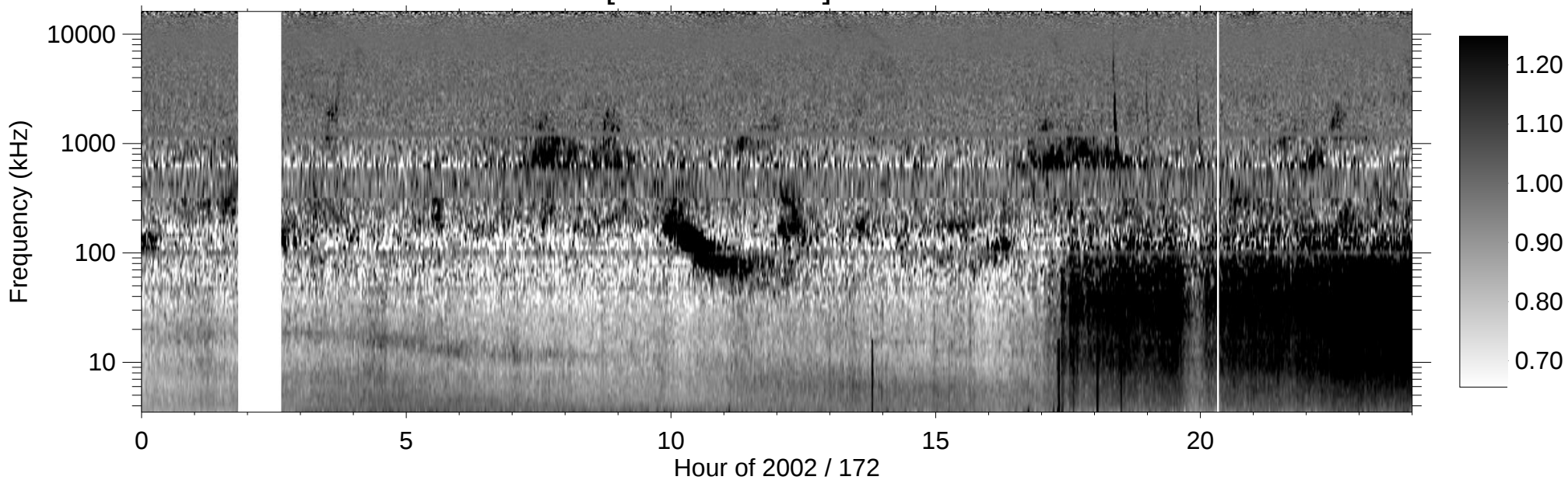
RPWS [ABCH1H2/Ex] (-B) 2002/06/21
