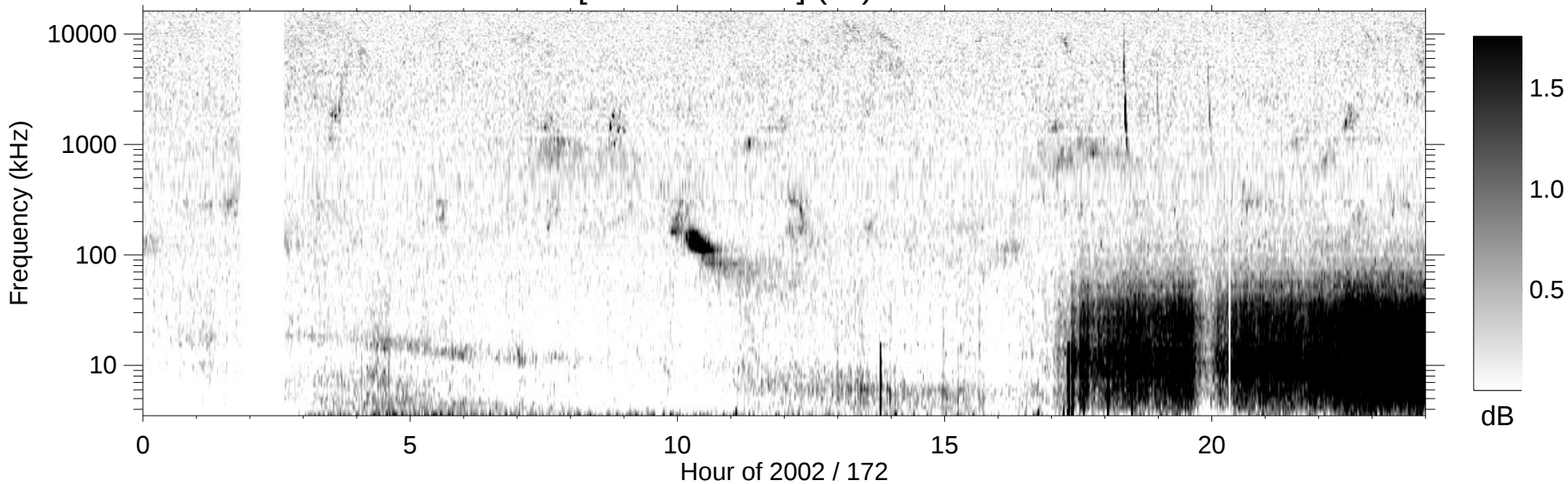
RPWS [ABCH1H2/Ex] (-B) 2002/06/21
