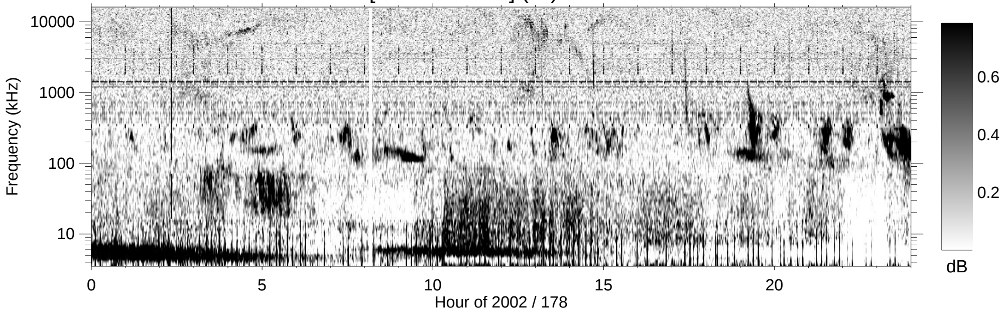
RPWS [ABCH1H2/Ex] (-B) 2002/06/27
