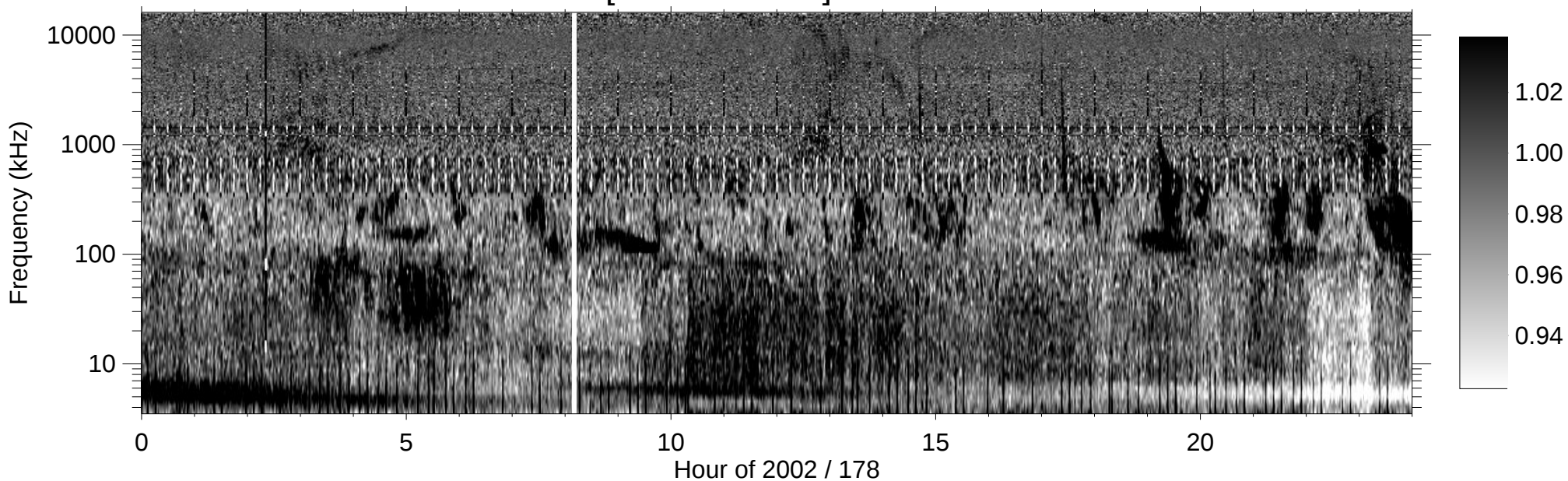
RPWS [ABCH1H2/Ex] (-B) 2002/06/27
