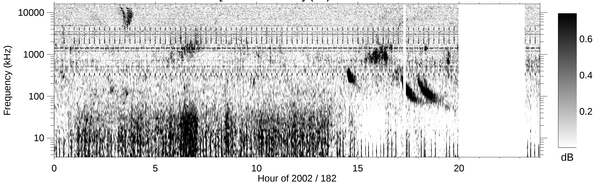
RPWS [ABCH1H2/Ex] (-B) 2002/07/01
