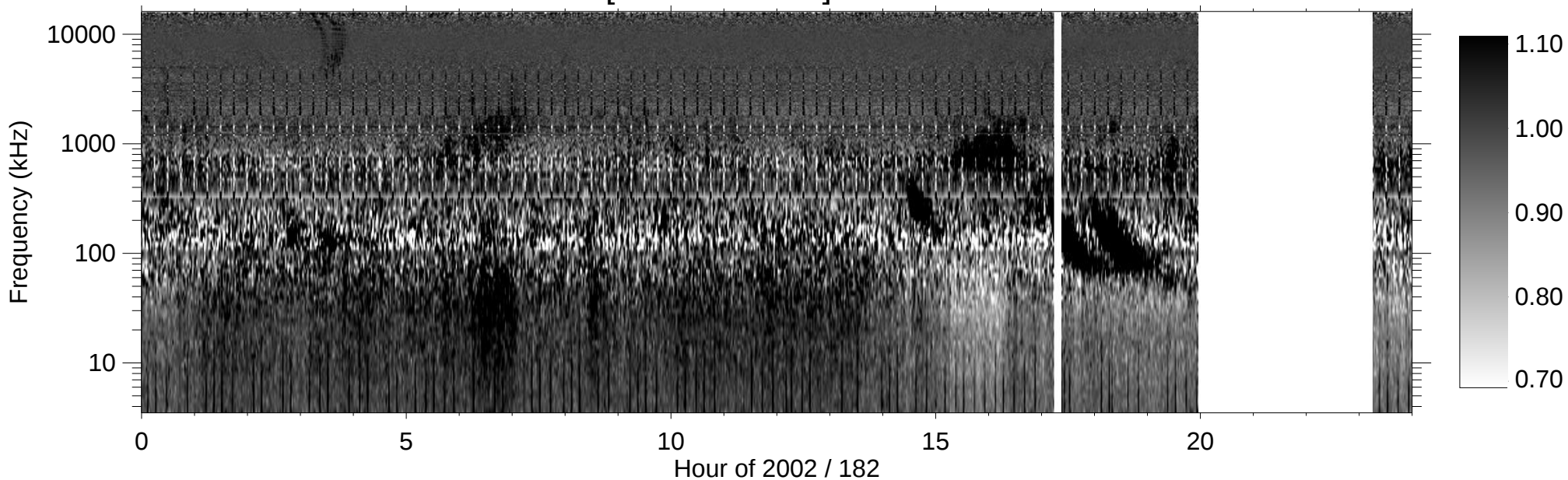
RPWS [ABCH1H2/Ex] (-B) 2002/07/01
