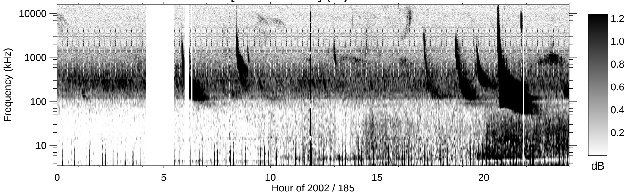
RPWS [ABCH1H2/Ex] (-B) 2002/07/04
