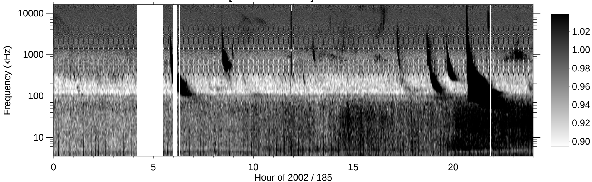
RPWS [ABCH1H2/Ex] (-B) 2002/07/04
