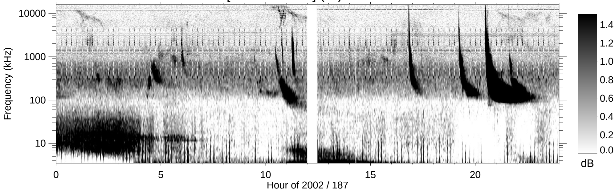
RPWS [ABCH1H2/Ex] (-B) 2002/07/06
