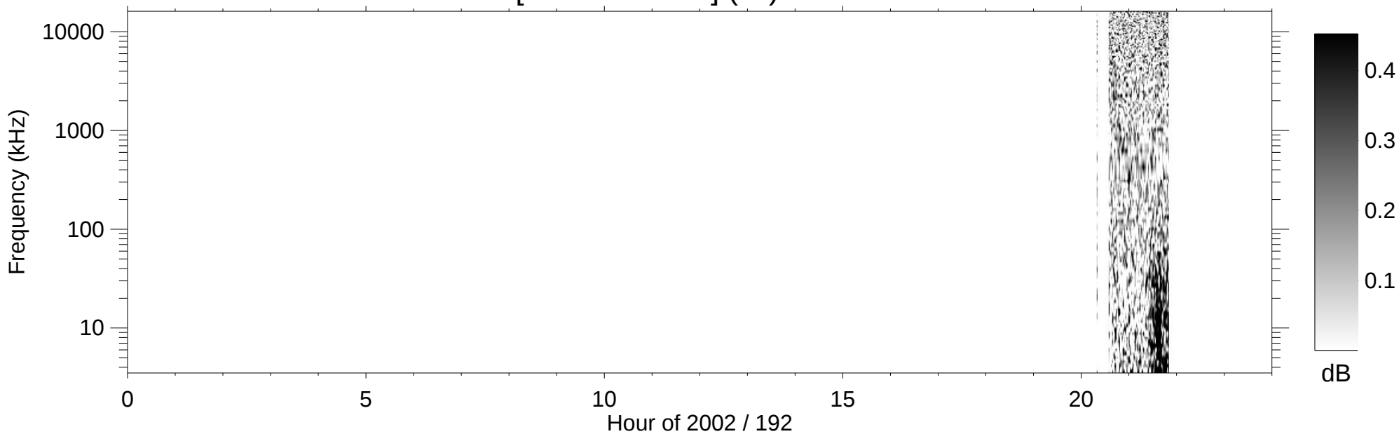
RPWS [ABCH1H2/Ex] (-B) 2002/07/11
