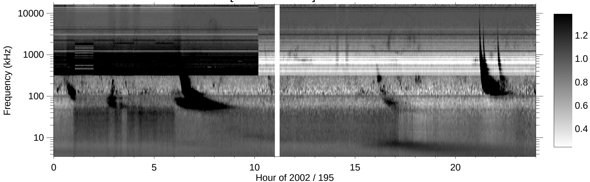
RPWS [ABCH1H2/Ex] (-B) 2002/07/14
