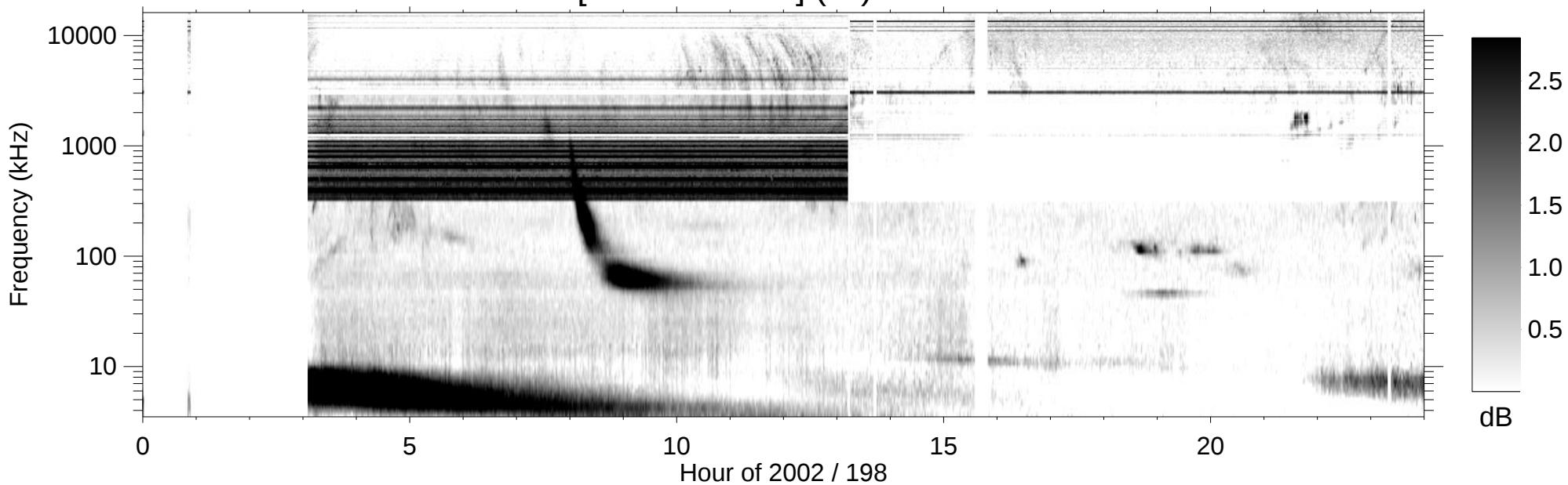
RPWS [ABCH1H2/Ex] (-B) 2002/07/17
