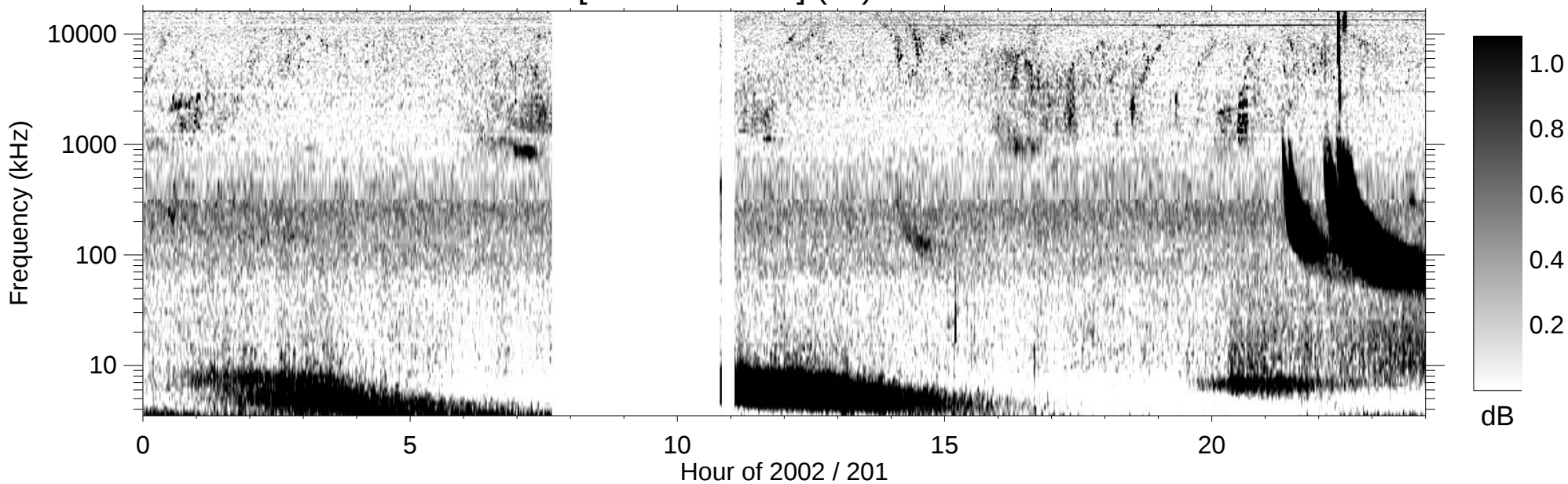
RPWS [ABCH1H2/Ex] (-B) 2002/07/20
