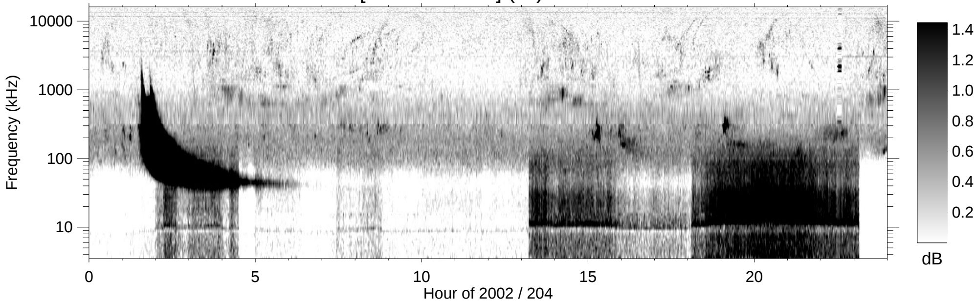
RPWS [ABCH1H2/Ex] (-B) 2002/07/23
