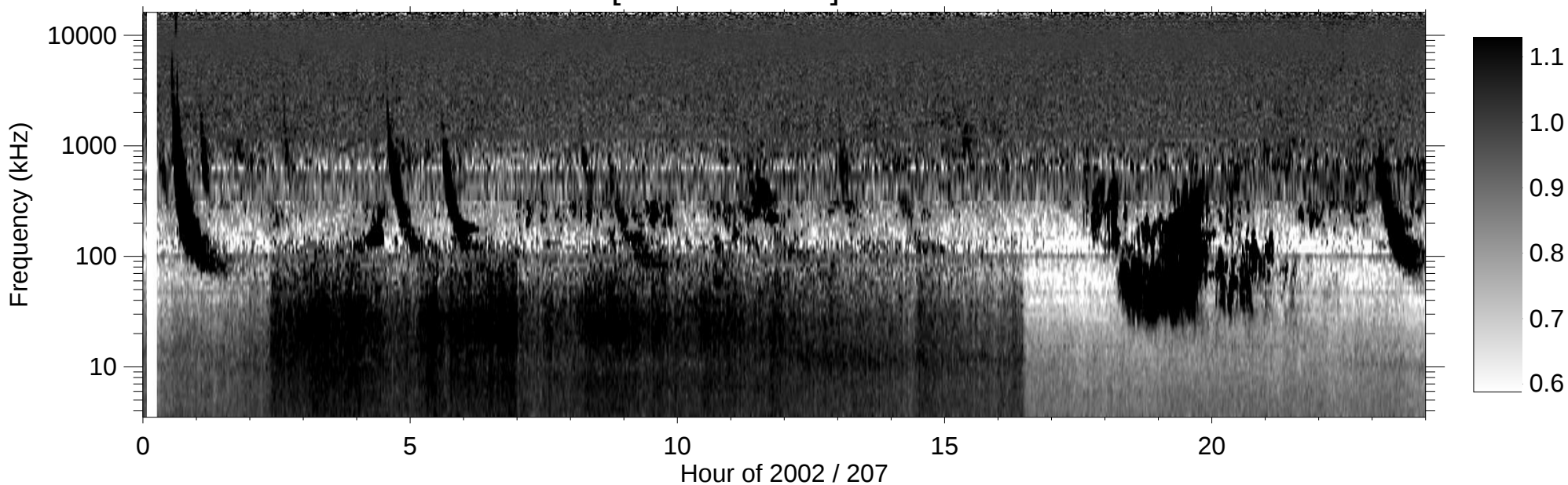
RPWS [ABCH1H2/Ex] (-B) 2002/07/26
