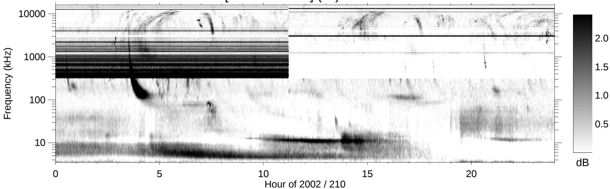
RPWS [ABCH1H2/Ex] (-B) 2002/07/29
