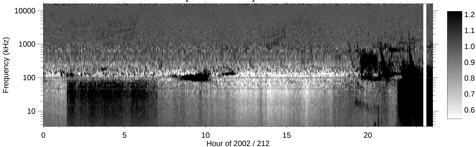
RPWS [ABCH1H2/Ex] (-B) 2002/07/31
