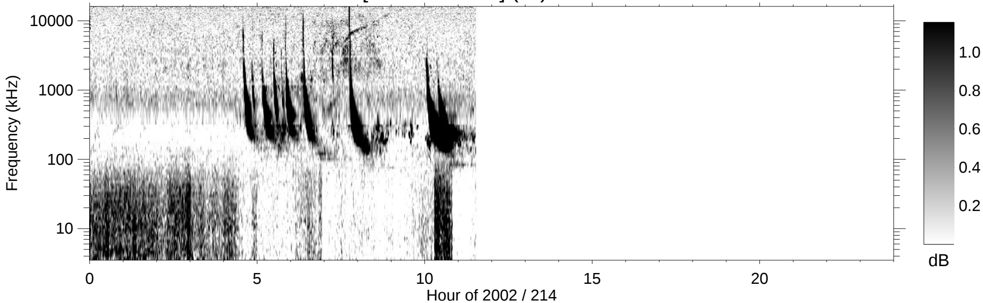
RPWS [ABCH1H2/Ex] (-B) 2002/08/02
