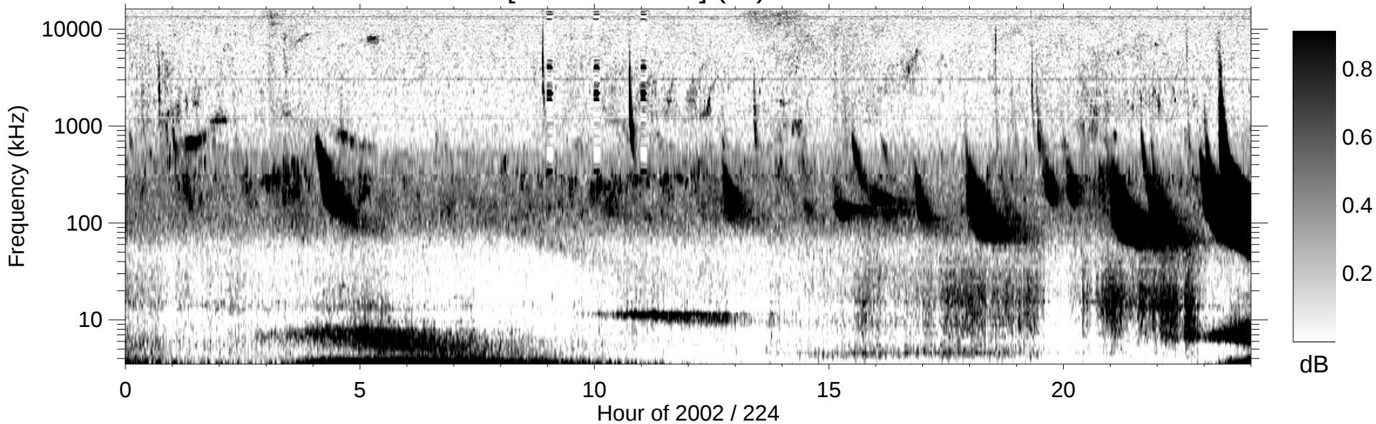
RPWS [ABCH1H2/Ex] (-B) 2002/08/12
