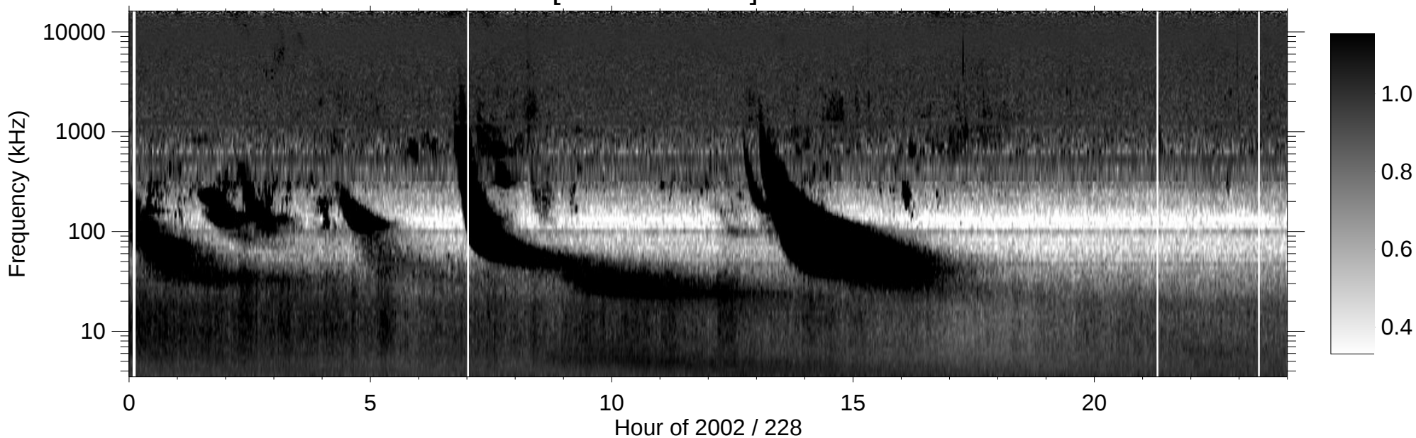
RPWS [ABCH1H2/Ex] (-B) 2002/08/16
