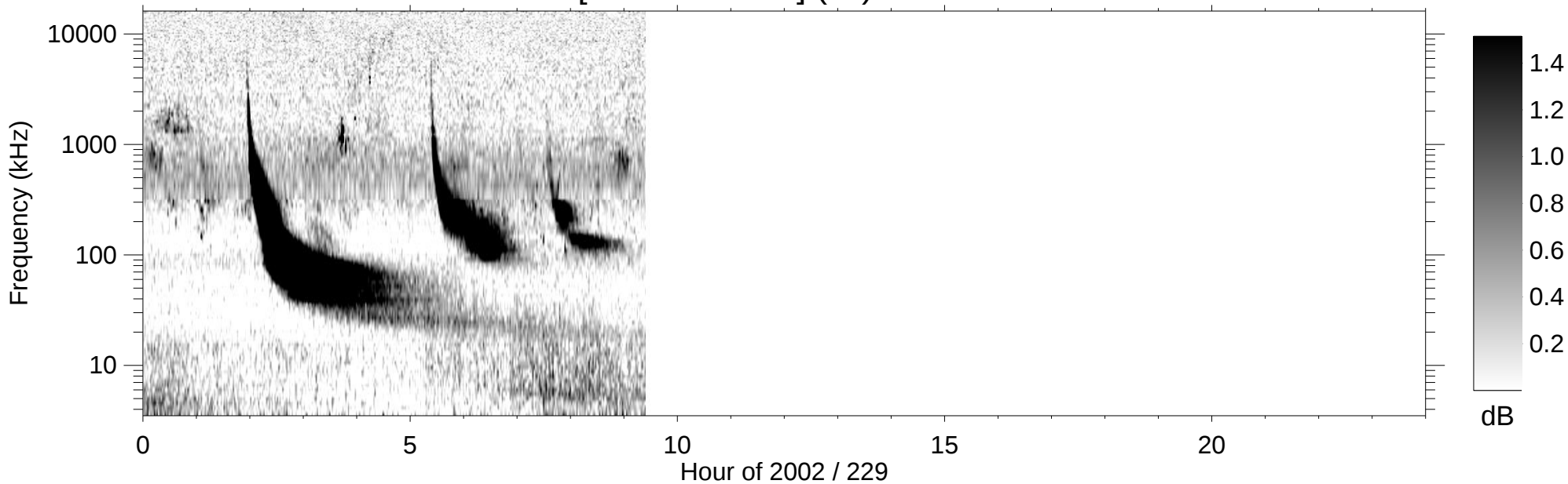
RPWS [ABCH1H2/Ex] (-B) 2002/08/17
