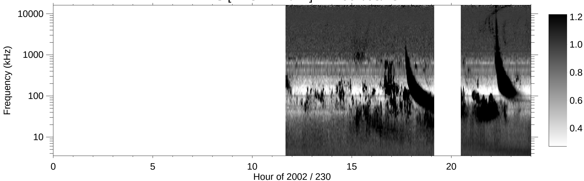
RPWS [ABCH1H2/Ex] (-B) 2002/08/18
