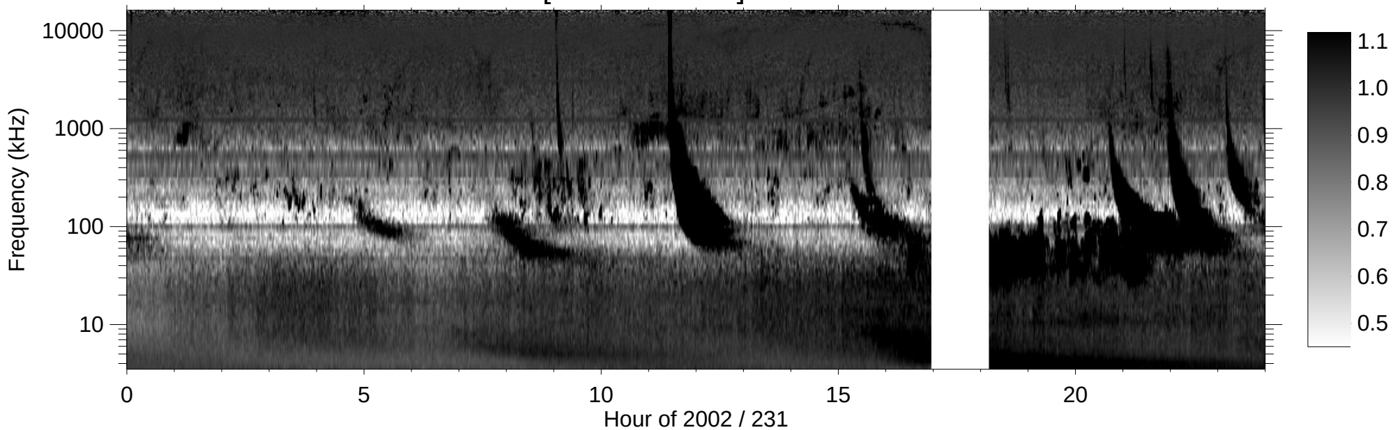
RPWS [ABCH1H2/Ex] (-B) 2002/08/19
