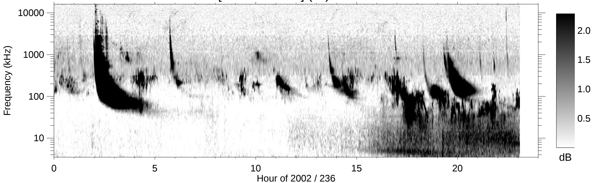
RPWS [ABCH1H2/Ex] (-B) 2002/08/24
