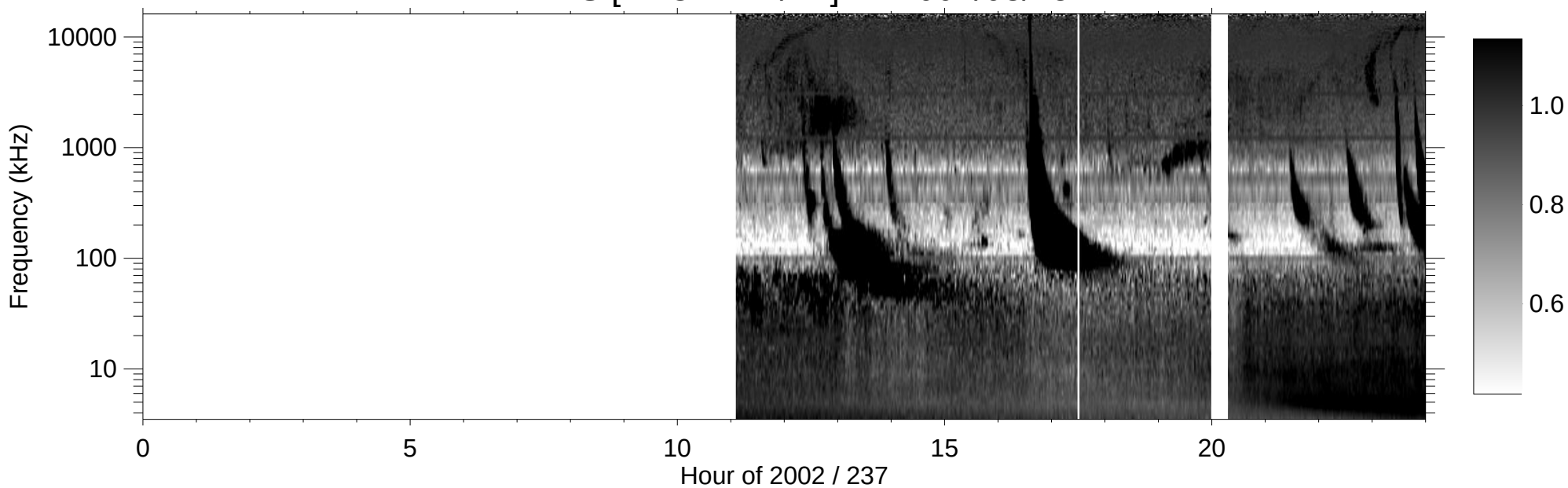
RPWS [ABCH1H2/Ex] (-B) 2002/08/25
