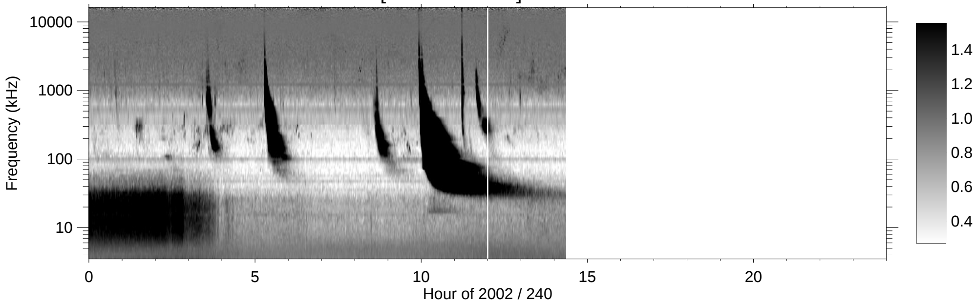
RPWS [ABCH1H2/Ex] (-B) 2002/08/28
