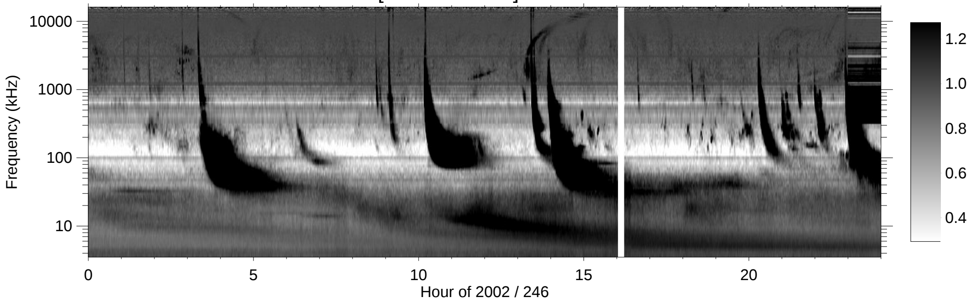
RPWS [ABCH1H2/Ex] (-B) 2002/09/03
