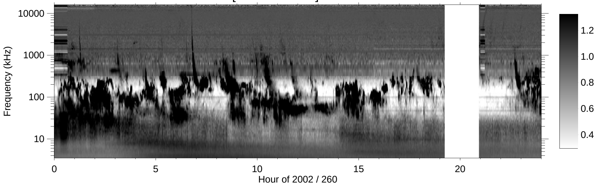
RPWS [ABCH1H2/Ex] (-B) 2002/09/17
