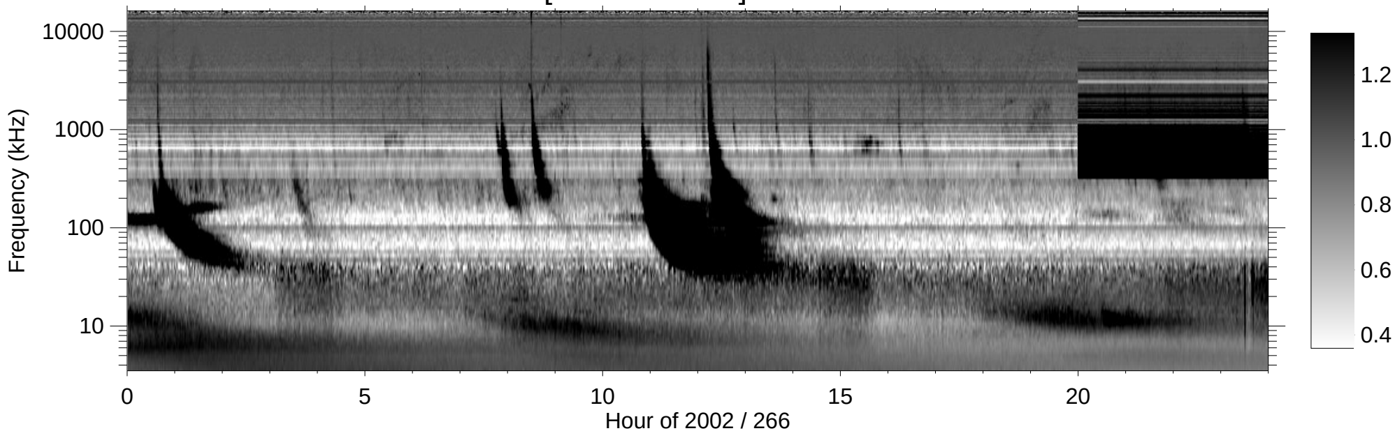
RPWS [ABCH1H2/Ex] (-B) 2002/09/23
