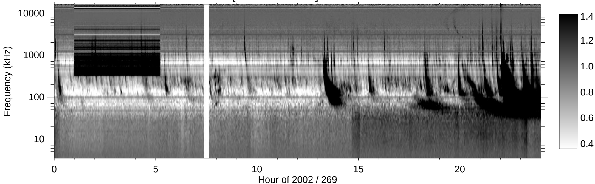
RPWS [ABCH1H2/Ex] (-B) 2002/09/26
