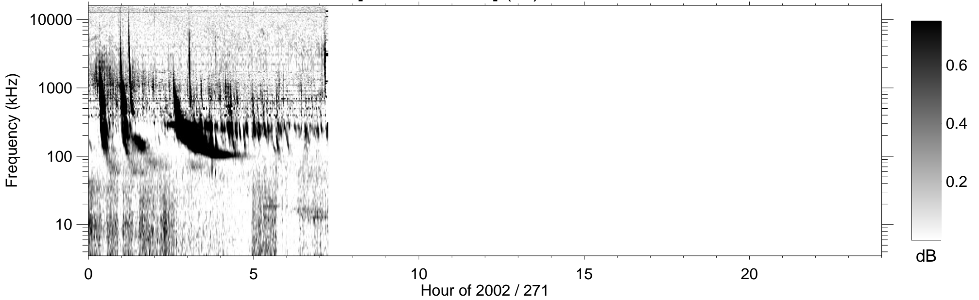
RPWS [ABCH1H2/Ex] (-B) 2002/09/28
