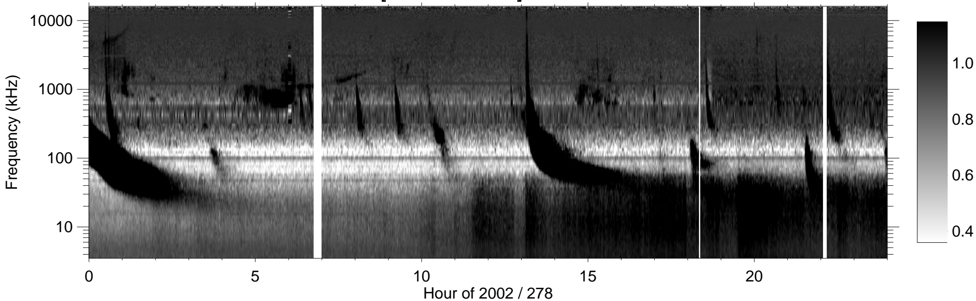
RPWS [ABCH1H2/Ex] (-B) 2002/10/05
