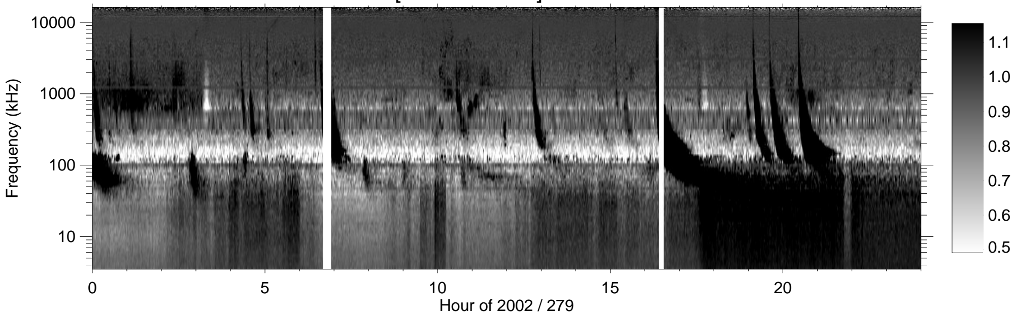
RPWS [ABCH1H2/Ex] (-B) 2002/10/06
