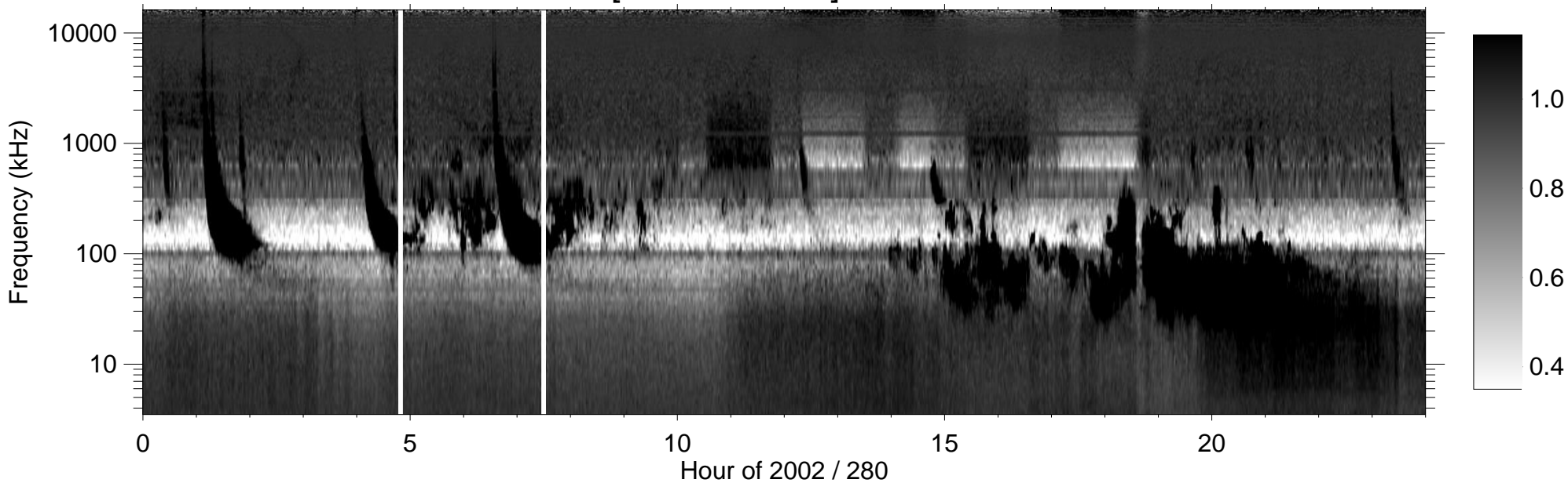
RPWS [ABCH1H2/Ex] (-B) 2002/10/07
