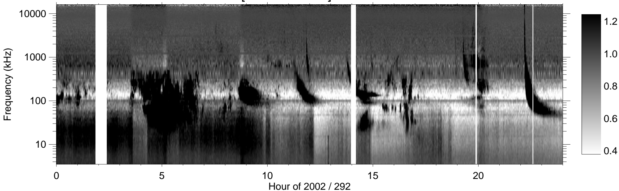
RPWS [ABCH1H2/Ex] (-B) 2002/10/19
