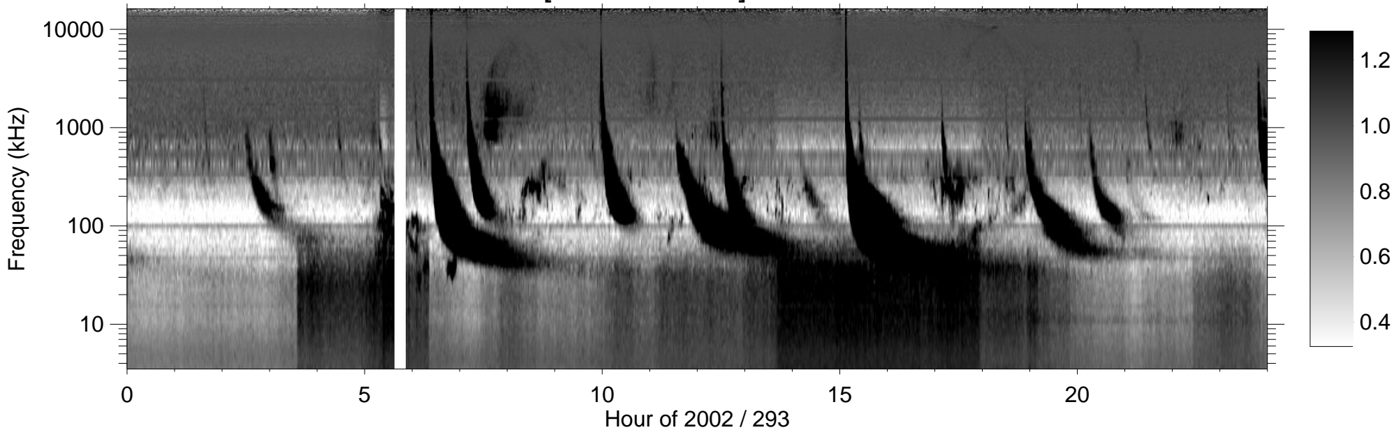
RPWS [ABCH1H2/Ex] (-B) 2002/10/20
