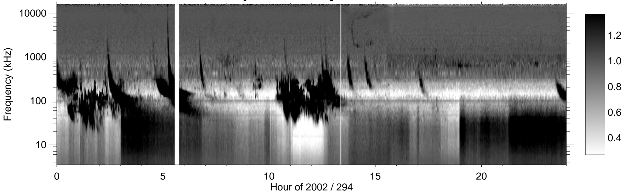
RPWS [ABCH1H2/Ex] (-B) 2002/10/21
