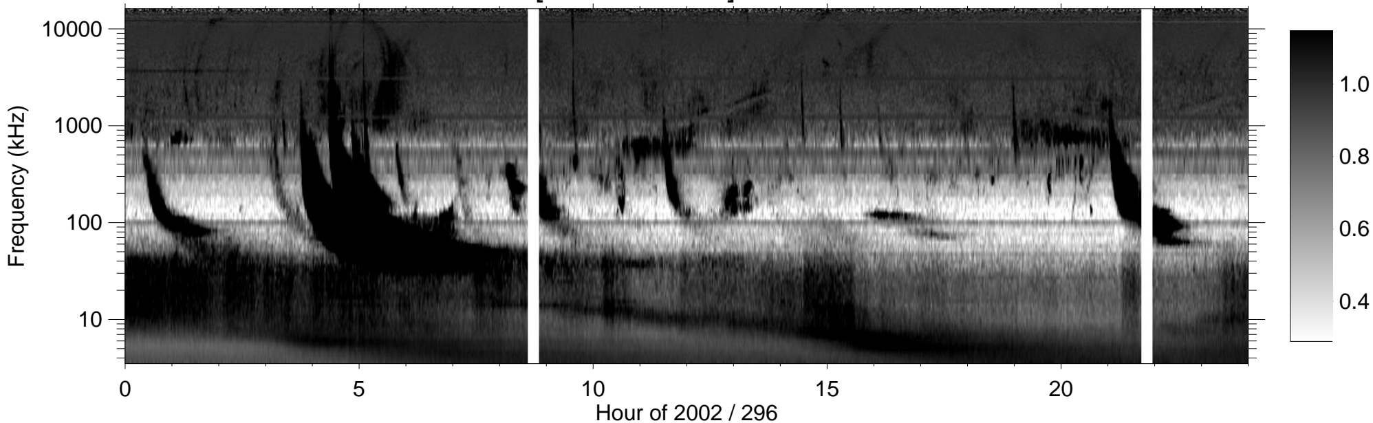
RPWS [ABCH1H2/Ex] (-B) 2002/10/23
