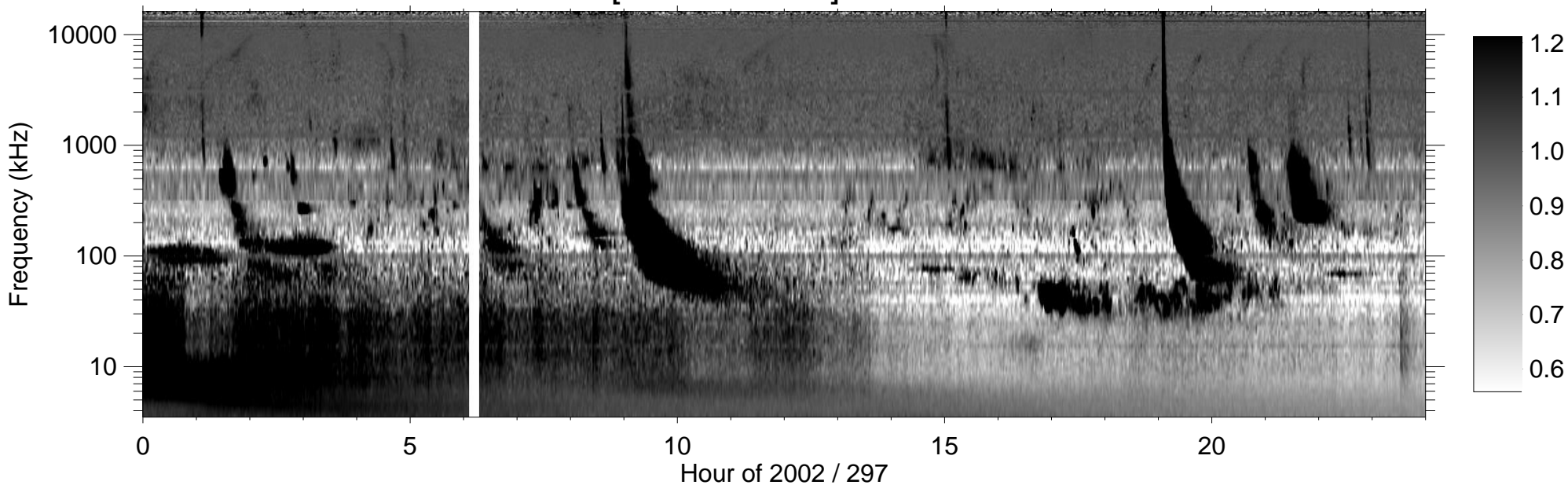
RPWS [ABCH1H2/Ex] (-B) 2002/10/24
