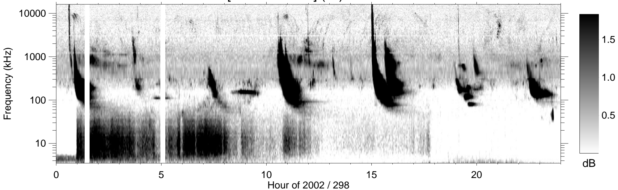
RPWS [ABCH1H2/Ex] (-B) 2002/10/25
