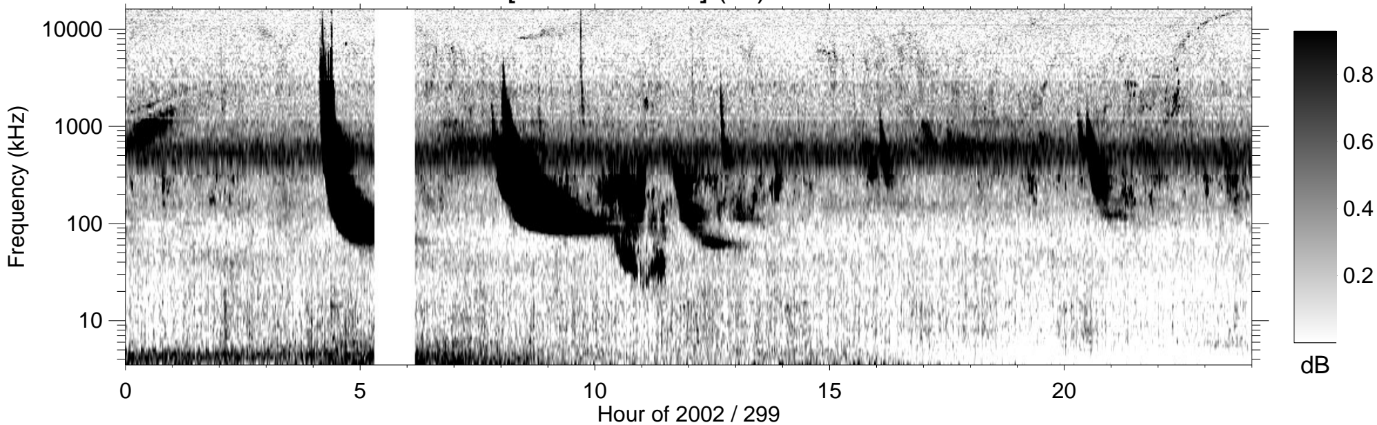
RPWS [ABCH1H2/Ex] (-B) 2002/10/26
