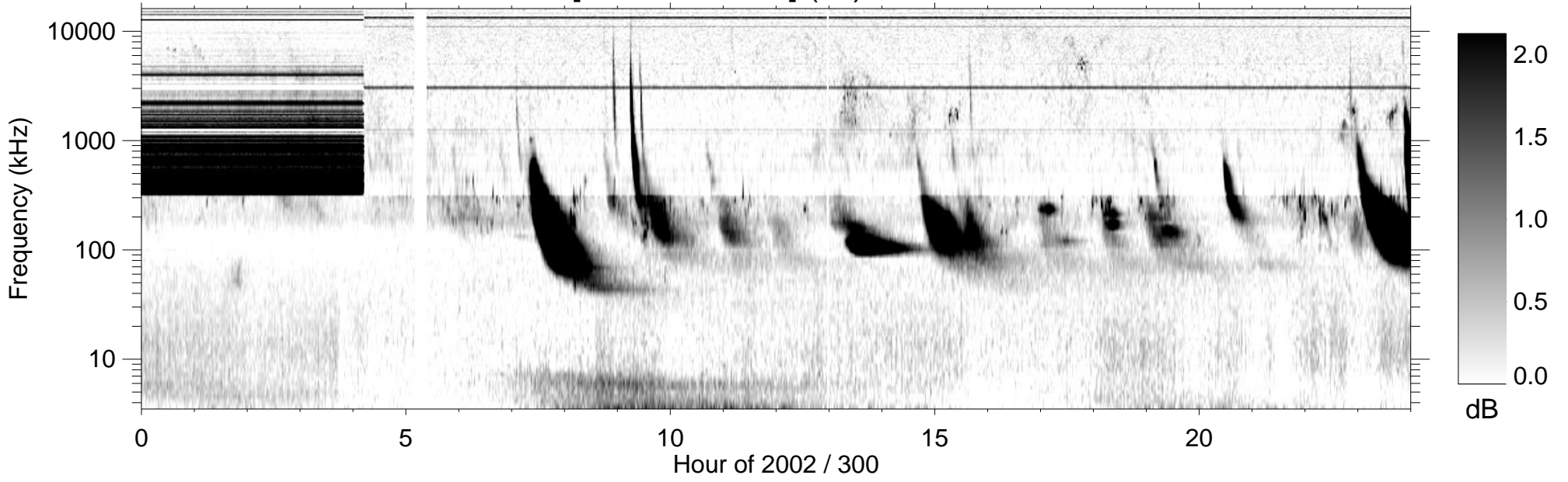
RPWS [ABCH1H2/Ex] (-B) 2002/10/27
